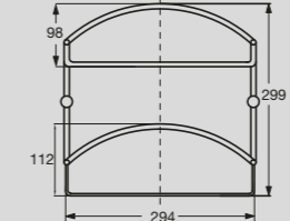
Solus Double Shelf System
