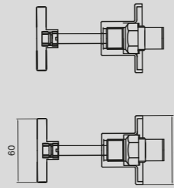
Solus Wall Top Assembly
