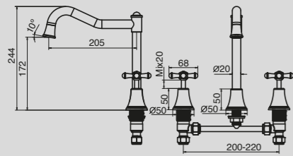
Canterbury English Hob Spa Set
