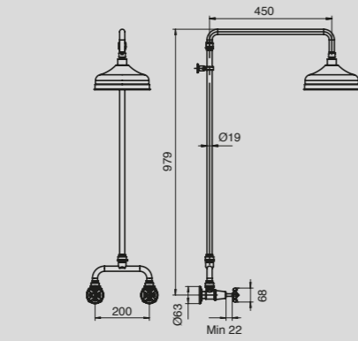
Canterbury Exposed Shower Set
