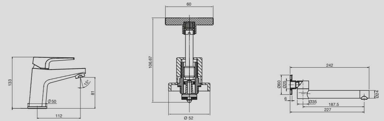
Solus MK2 Basin Mixer
