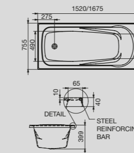
Solus MK2 Rectangular Santai Spa
