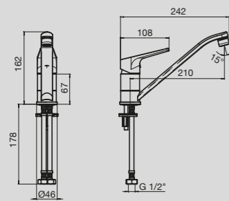
Solus MK3 Standard Sink Mixer
