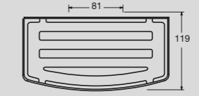
Solus Metal Shower Basket
