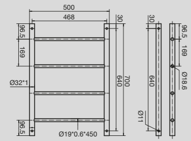
Solus MK2 Heated Towel Rail 700mm h x 500mm w
