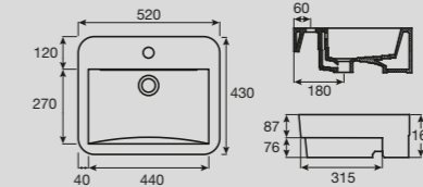
Solus Semi Recessed Basin 520 x 430mm
