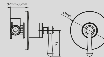
Canterbury Shower/Bath Mixer
