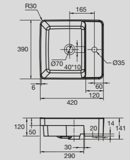
Domaine Semi Recessed Basin
