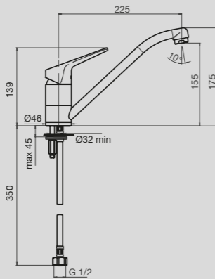
Solus MK2 Standard Sink Mixer
