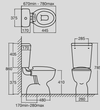
Solus Square Link Toilet Suite
