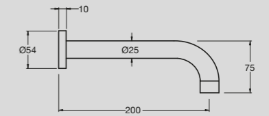
Solus Curved Bath Outlet
