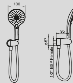
Domaine 3 Function Hand Shower
