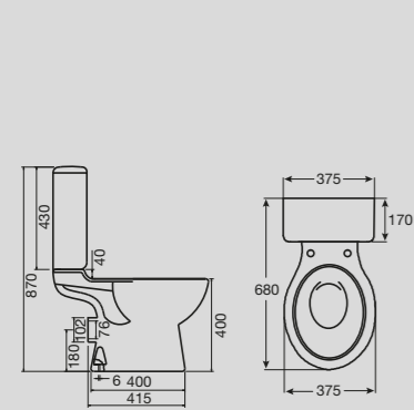
Solus Round Close Coupled P Trap Toilet Suite
