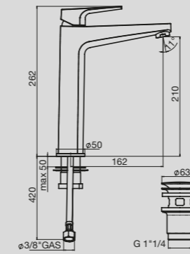
Solus MK2 Extended Basin Mixer
