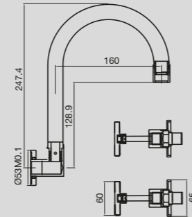
Solus Wall Sink Set
