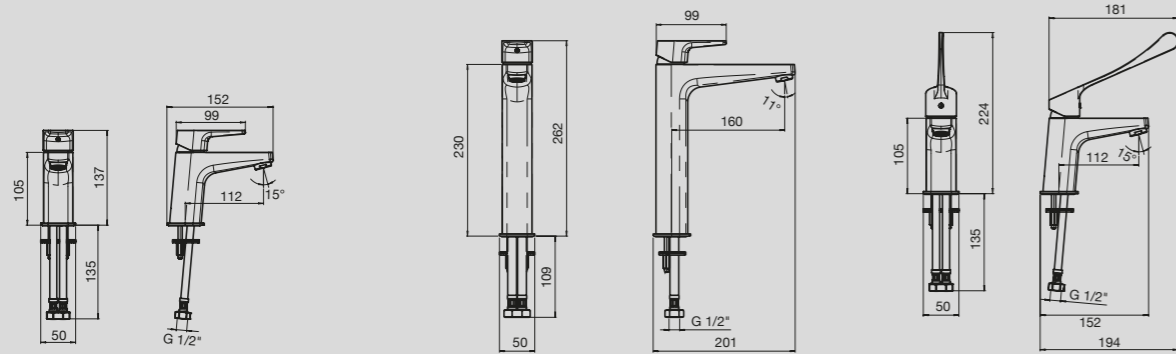
Solus MK3 Basin Mixer
