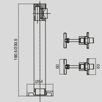
Solus Bath Set
