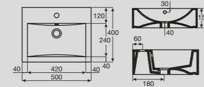
Solus Counter Basin
