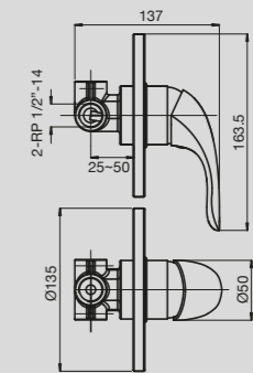
Bristol MK2 Shower Mixer
