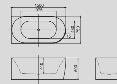
Solus 1500 Back to Corner Freestanding Bath
