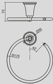
Canterbury Towel Ring
