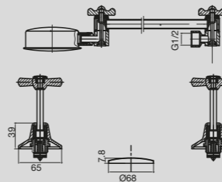
Bristol Shower Set
