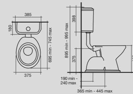
Canterbury Low Level Toilet Suite
