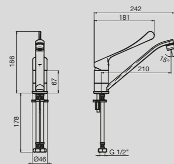
Solus MK3 Extended Lever Standard Sink Mixer
