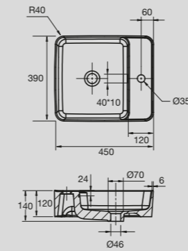
Domaine Counter Basin
