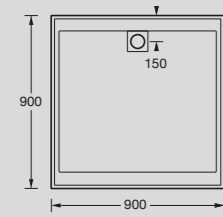
Solus 900 x 900mm Shower Base
