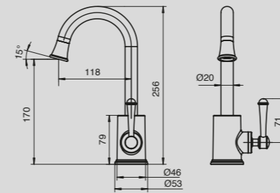
Canterbury Basin Mixer
