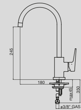
Solus MK2 Gooseneck Sink Mixer
