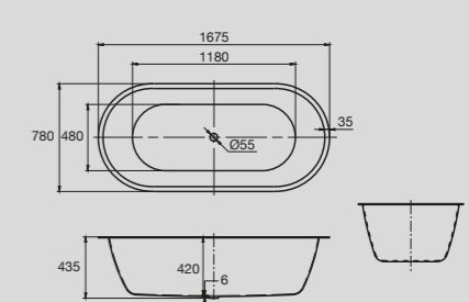
Solus Oval Inset Bath
