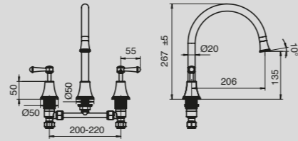
Canterbury Hob Spa Set Lever
