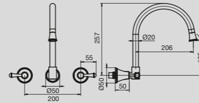
Canterbury Wall Sink Set Lever
