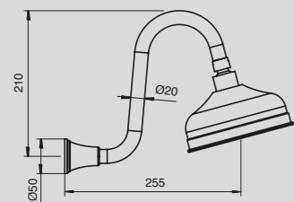
Canterbury Shower Arm & Rose
