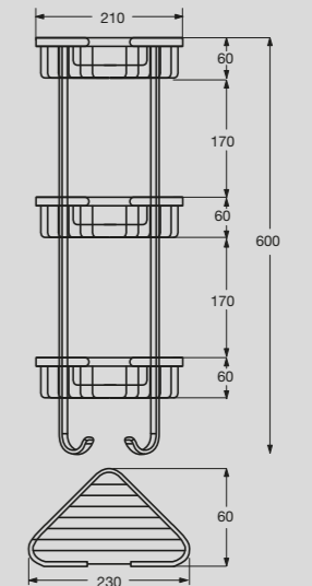
Solus Corner Basket System
