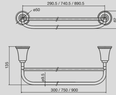
Canterbury Double Towel Rail 300mm / 750mm / 900mm
