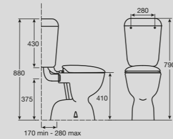
Solus Round Link Toilet Suite
