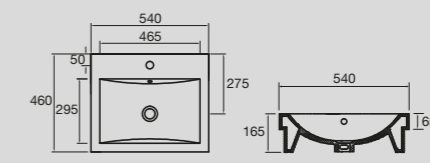
Solus Semi Inset Basin 540 x 460mm
