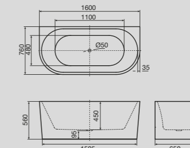
Solus Back to Wall Freestanding Bath
