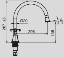
Canterbury Hob Spa Outlet
