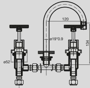
Solus Basin Set
