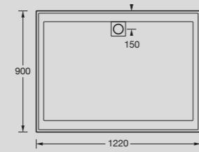
Solus 1200 x 900mm Shower Base
