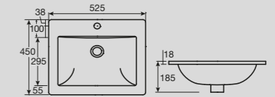
Solus Vanity Basin 525 x 450mm
