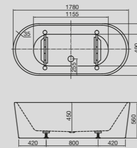
Solus 1780 Freestanding Bath
