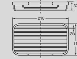
Solus Large Rectangular Wire Basket
