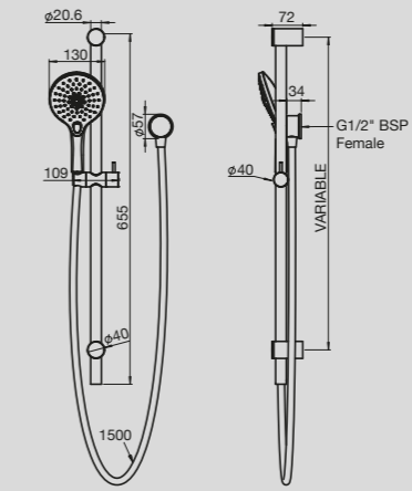
Domaine 3 Function Brass Rail Shower
