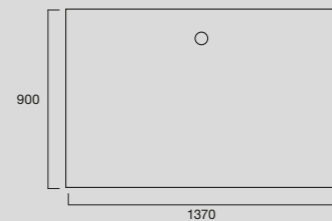
Bristol Torbex MK2 1370 x 900mm Rectangle Shower Base
