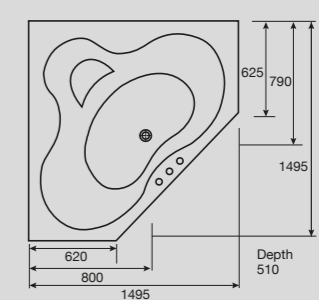
Solus MK2 Corner Santai Spa
