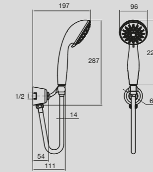
Bristol Hand Shower with Wall Bracket
