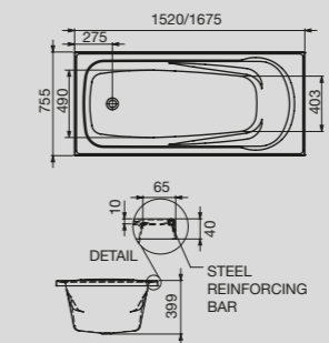
Solus MK2 Rectangular Inset Bath
