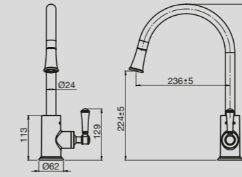
Canterbury Pull Out Sink Mixer with Porcelain Handles
