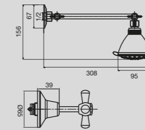
Bristol Deluxe Shower Set
