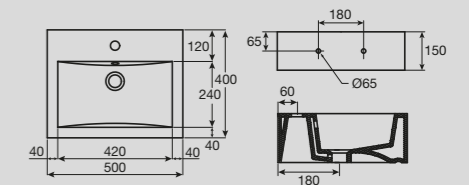
Solus Wall Basin 500 x 400mm
