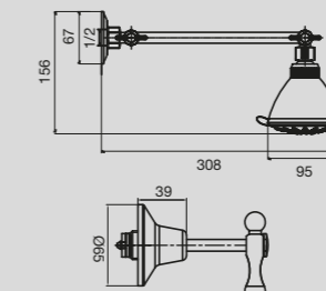
Bristol Deluxe Shower Set Lever Handle
