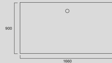
Bristol Torbex MK2 1660 x 900mm Rectangle Shower Base
