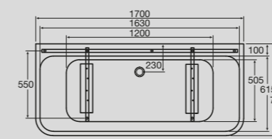
Domaine Back to Wall Freestanding Bath
