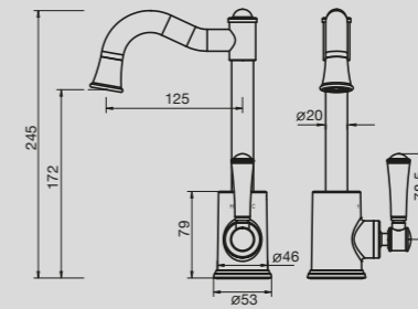
Canterbury English Basin Mixer
