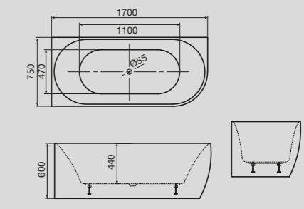
Solus 1700 Back to Corner Freestanding Bath
