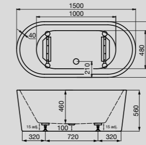
Solus 1500 Freestanding Bath
