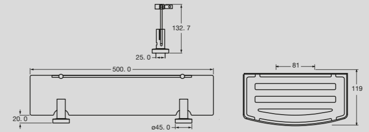
Solus MK2 Glass Shelf
