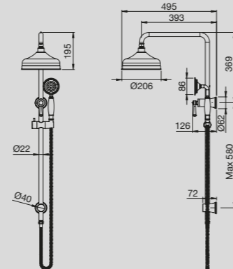
Canterbury Twin Rail Shower
